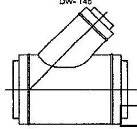
Y-BRANCH DW- Y45
